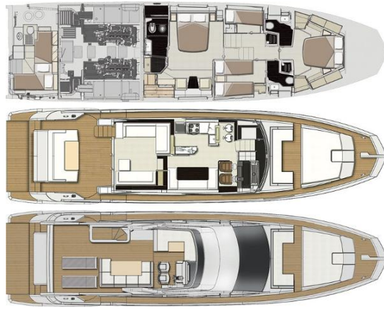
Deck Plans
